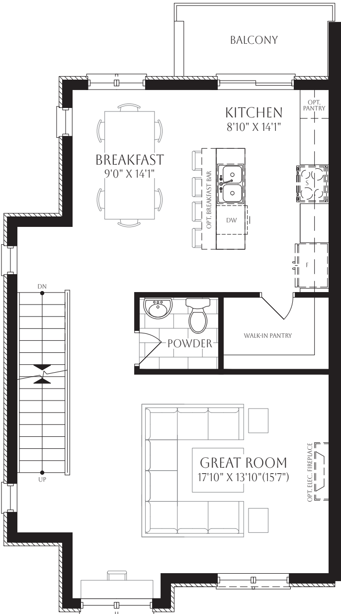
SECOND FLOOR
